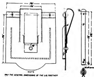
Figs. 4839-4842. Standard Journal Box Lid and Pin for Journal, 4\frac{1}{4} in. x 8 in. Plate 7.
